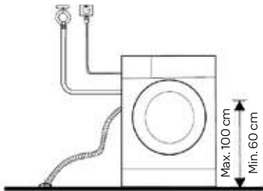
1. Put the water discharge hose in a floor drain.
